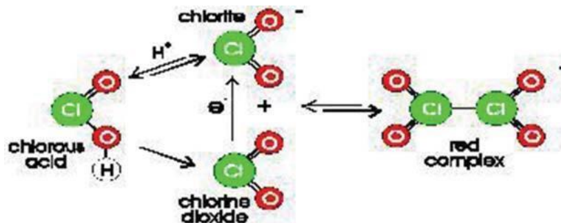
Fig. 57: Oxidation Redox
